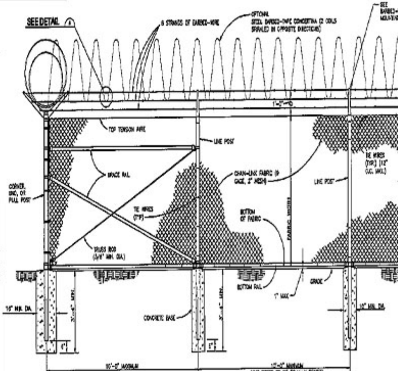
CHAIN-LINK SECURITY FENCE DETAIL 10 TO SCALE
