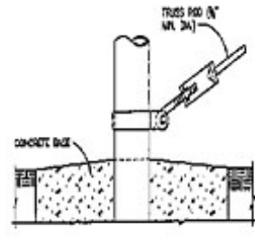
TRUSS ROD AND BAND
