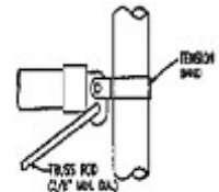
BRACE RAIL CLAMP DETAIL
