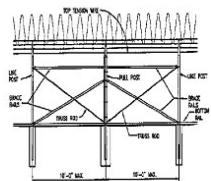
BRACE PANEL DETAIL 10 TO SCALE
