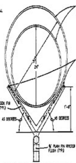
BARBED-TAPE MOUNTING DETAIL 10 TO SCALE
