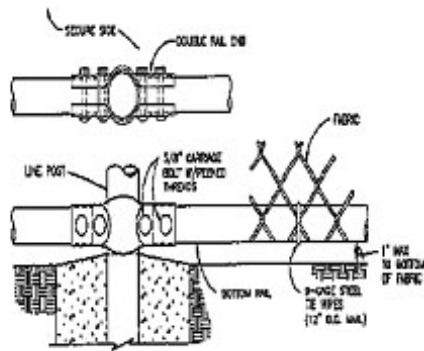
BOTTOM RAIL DETAILS 10 TO SCALE
