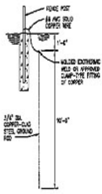
GROUNDING DETAIL 10 TO SCALE
